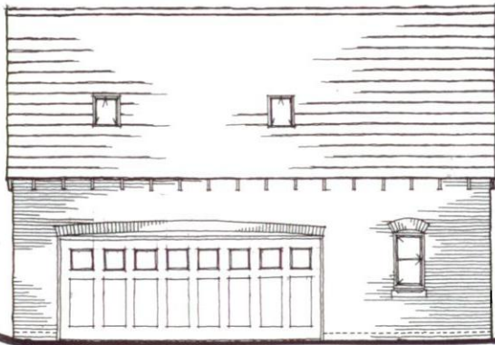
PROPOSED FRONT ELEVATION TO GARAGE.
